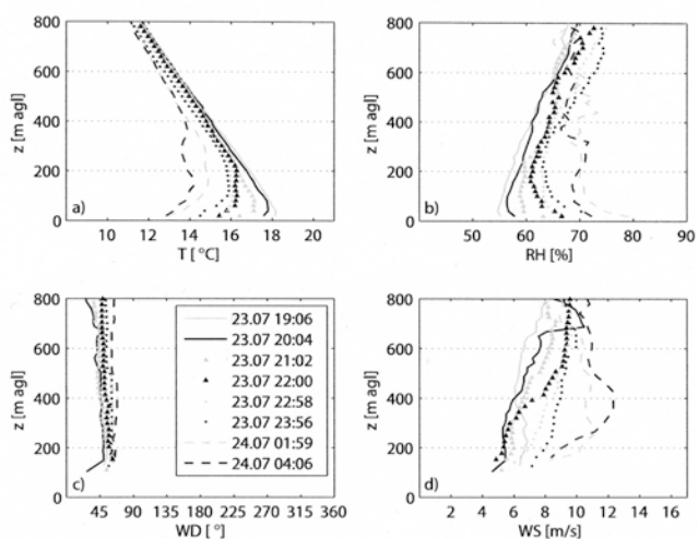
Figure 7: Example for the development of a stable nocturnal boundary layer. Airfield Coburg Steinrücken, 50.23°N and 10.99°E, 23./24.07.2008.
